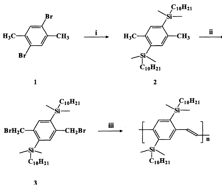
Scheme 2. Synthetic route for BDDMS-PPV. Reagents and conditions: i) Mg/THF, \text{Me}_2\text{SiC}_{10}\text{H}_{21}\text{Cl} ; ii) NBS/benzene/BPO/ h\nu ; iii) \text{KOBu}^t /THF.
